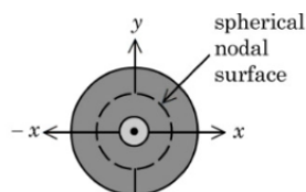
Figure 1. electron probability density for 2s orbital
