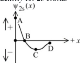
Figure 2. wave function for 2s orbital
