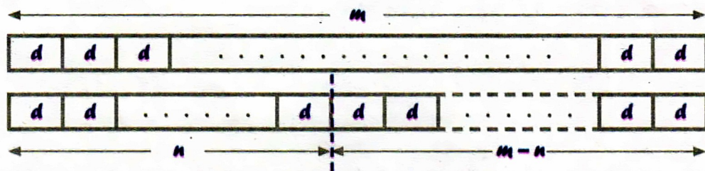
Fig. 11.1: Justification for Euclid's gcd algorithm
