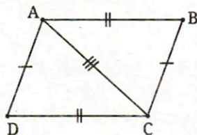
Fig. 12.7: Converse to (a)
