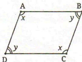
Fig. 12.8: Converse to (b) 2(x + y) = 360^\circ
