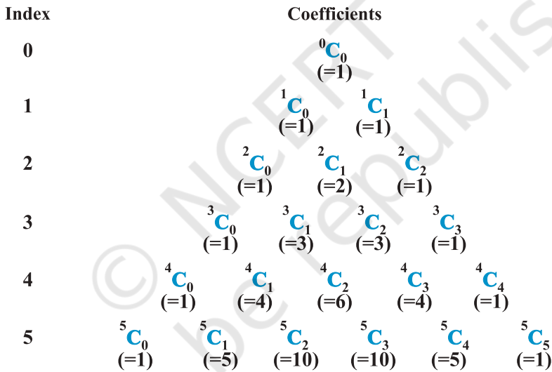
Fig 8.3 Pascal's triangle
